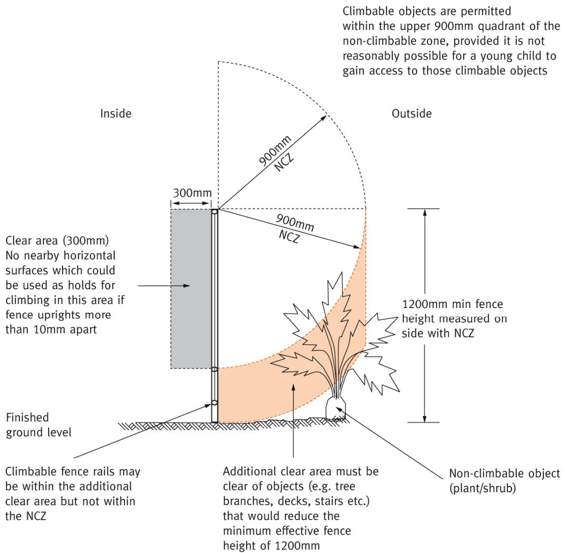
Figure 6 1200mm min high fence NCZ on outside Acceptable
